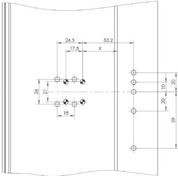
2 - WINGS - TOOLING IN PROFILE
