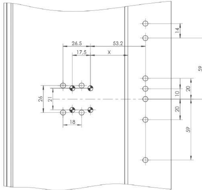
3 - WINGS - TOOLING IN PROFILE
